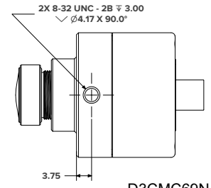
D3CMC69N Units: mm
