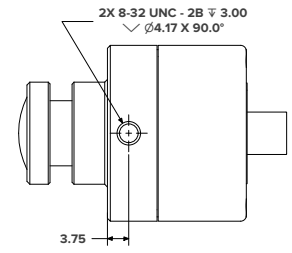
D3CMC52N Units: mm
